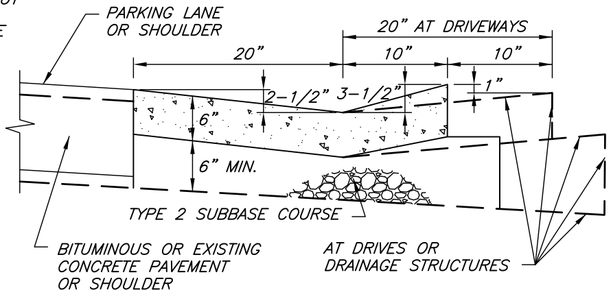
GUTTER SECTION
